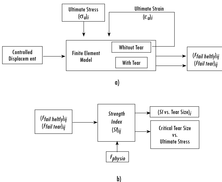
Figure 1. (A) Methodology used to estimate the forces needed to enlarge a tear. (B) Estimation of the relationships between the Strength Index ( SI ) and Critical Tear Size ( CTS ) with ultimate stress and tear size
