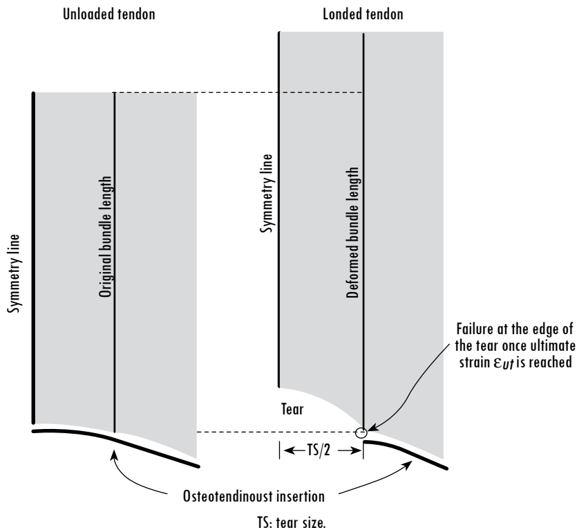
Figure 2. Failure of the tear edge fiber bundle at tendon ultimate strain ( \epsilon_{ut} ). The 2D finite element model of the healthy supraspinatus tendon was implemented to estimate the corresponding ultimate strain for the previously reported ultimate stress (range) of the supraspinatus tendon
