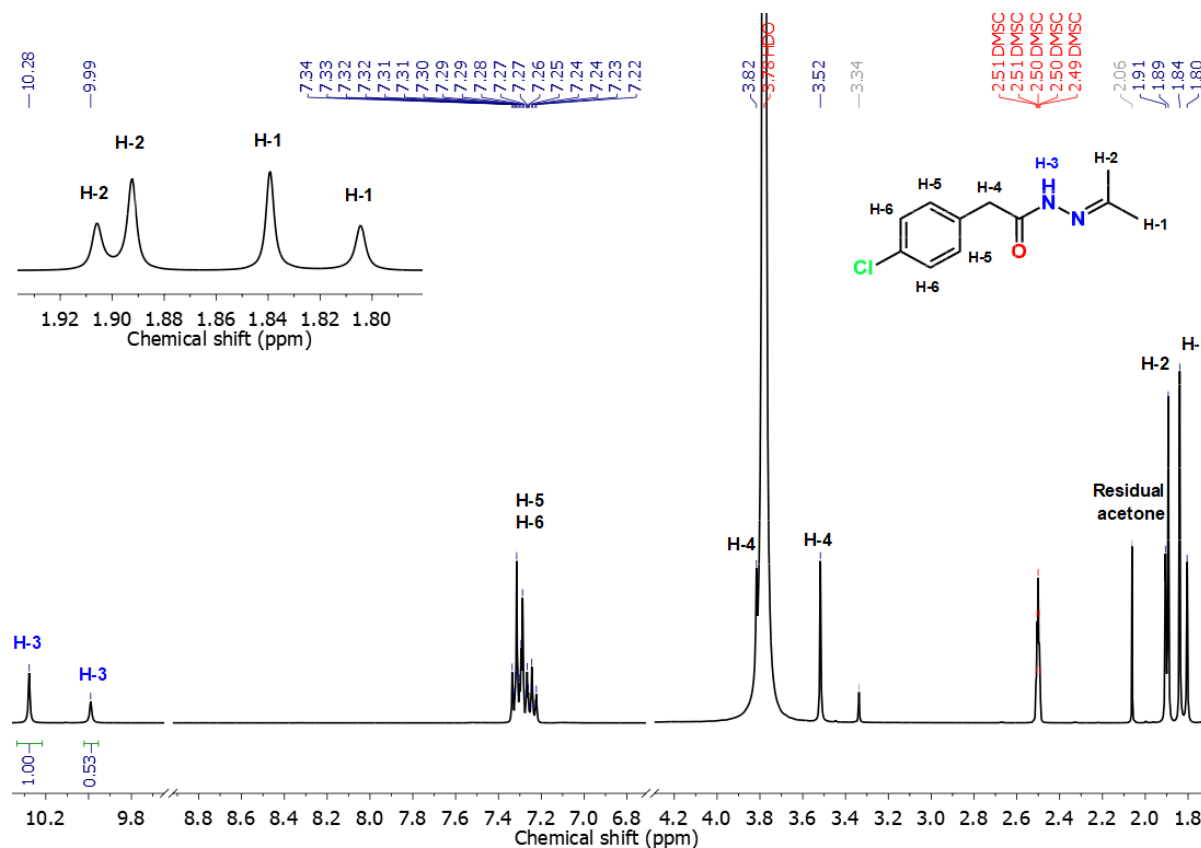
Figure 1. 1 H spectrum of 2-(4-clorophenyl)-N'-(propan-2-ylidene) acetohydrazide.
