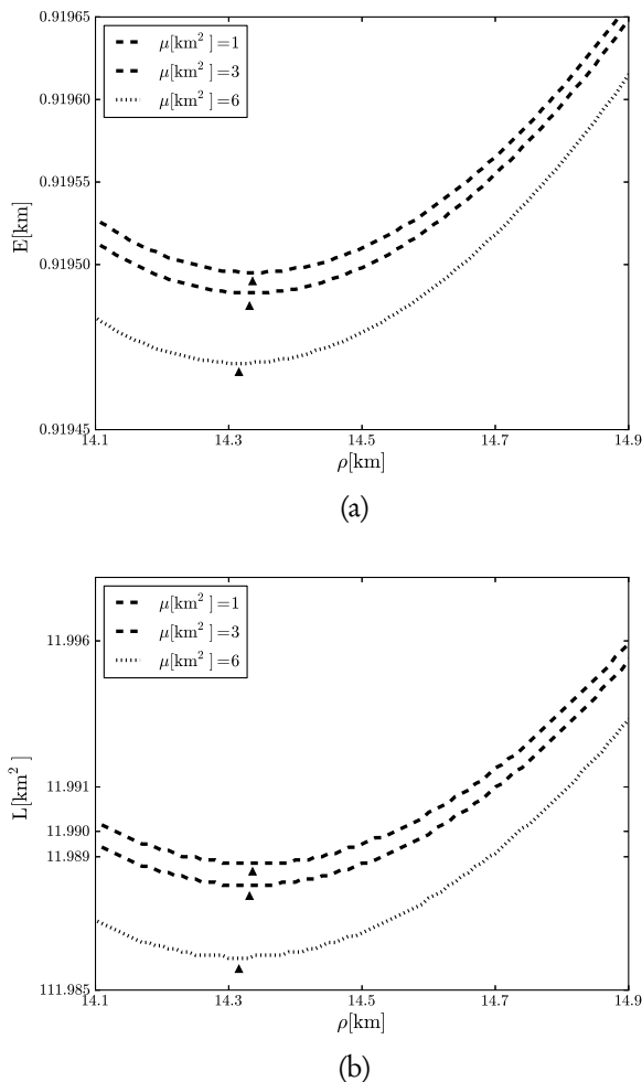
Fig. 4. Energy (a) and angular momentum (b) of a test particle at the ISCO radius versus magnetic dipole parameter \mu given by the PRS solution. We can see that reduction of the energy and angular momentum of the particle while the the magnetic dipole of the star is increased.
