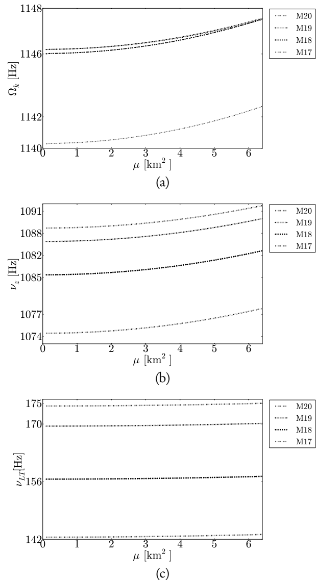
Fig. 2. Keplerian frequency (a), nodal precession frequency (b) and, Lense-Thirring frequency (c) as a function of the \mu parameter. All the frequencies increase for increasing \mu .
