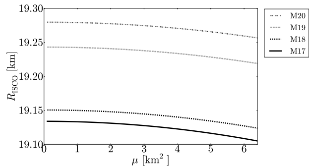
Fig. 1. ISCO radius as a function of magnetic dipole parameter \mu . The physical parameters for the star correspond to the models M17-M20 listed in Table 1. An increase of \mu leads to a decrease of the ISCO radius.
