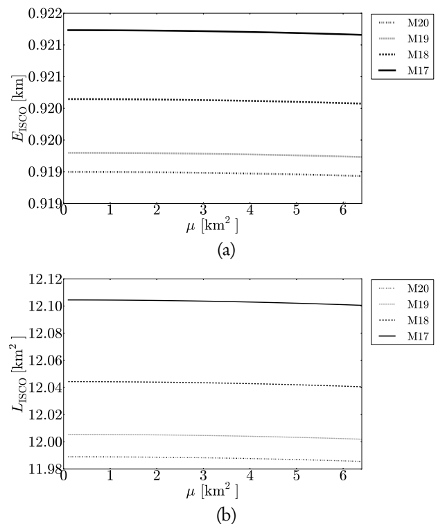
Fig. 3. Energy (a) and angular momentum (b) of a test particle at the ISCO radius versus magnetic dipole parameter \mu given by the PRS solution. We can see that reduction of the energy and angular momentum of the particle while the the magnetic dipole of the star is increased.
